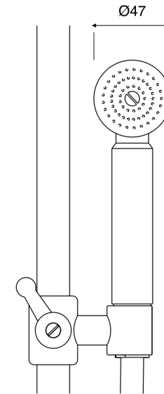
Hand shower and sliding holder
